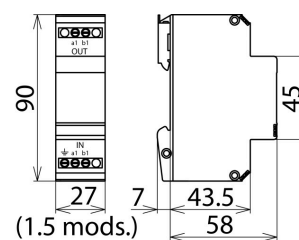
Dimension drawing BVT TC
